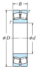
圆柱孔
